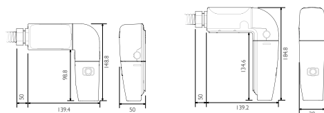
Horizontal 90 Degree Print Head Installation Dimensions
