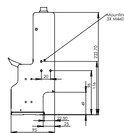
Standard Print Head
