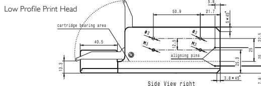
Low Profile Print Head
